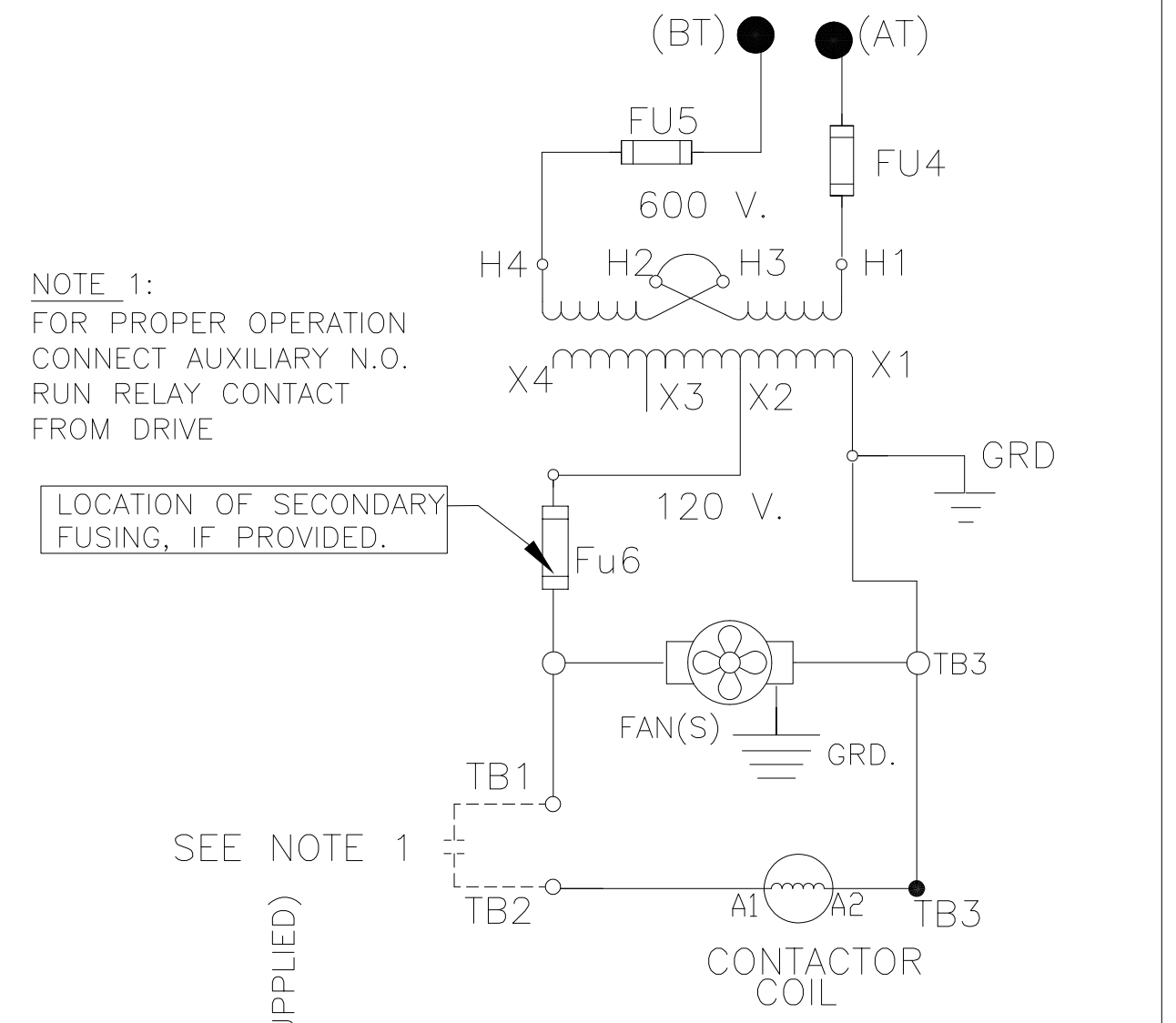
CONTROL CONNECTIONS WITH FAN(S)
