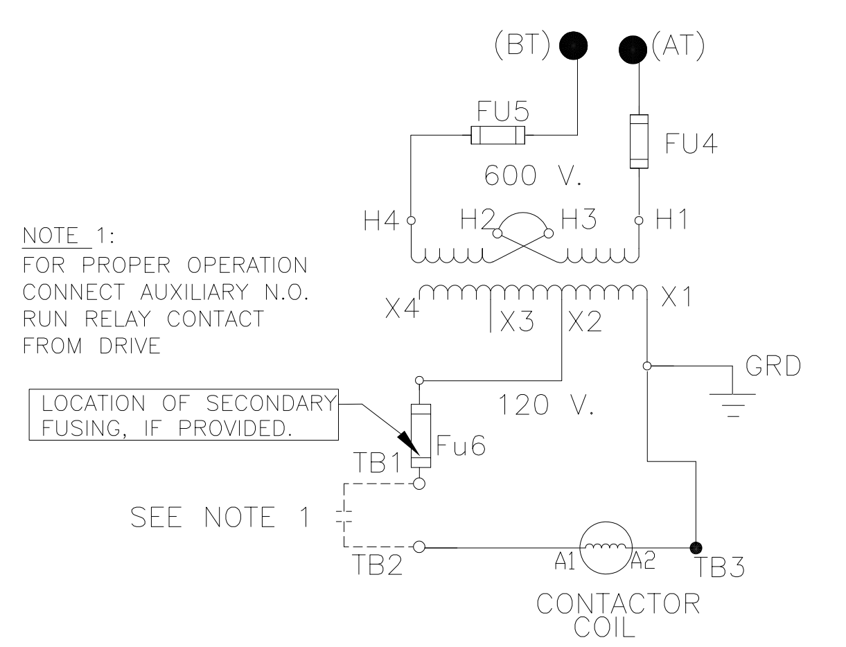
CONTROL CONNECTIONS WITHOUT FAN(S)
