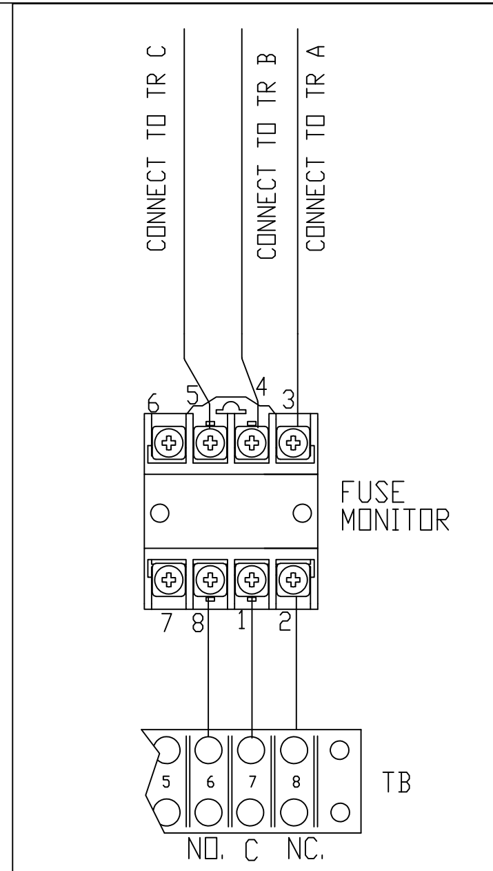
TERMINAL BLOCK ON PANEL
