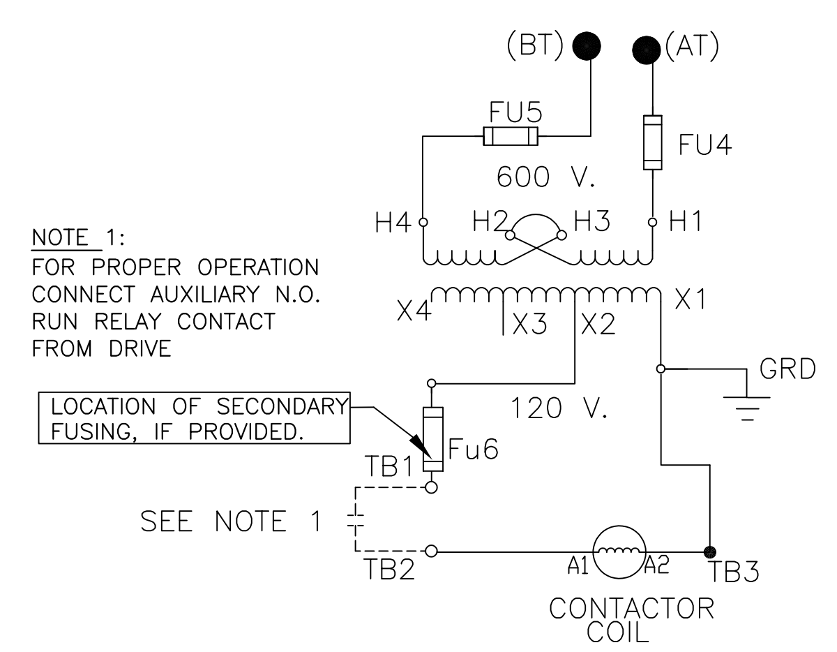
CONTROL CONNECTIONS WITHOUT FAN(S)
