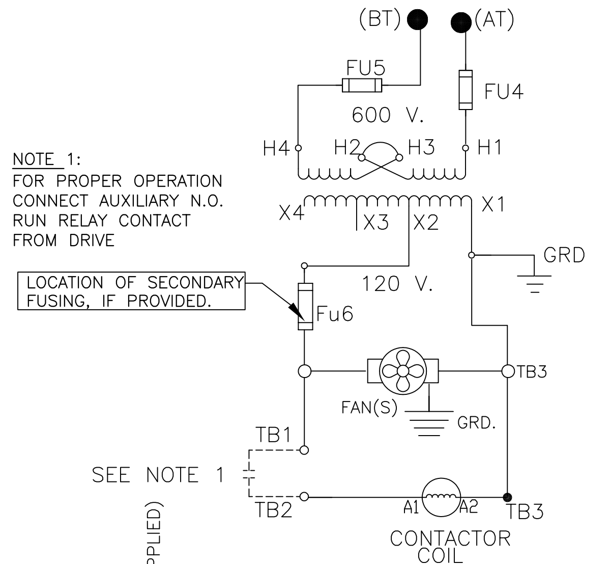
CONTROL CONNECTIONS WITH FAN(S)
