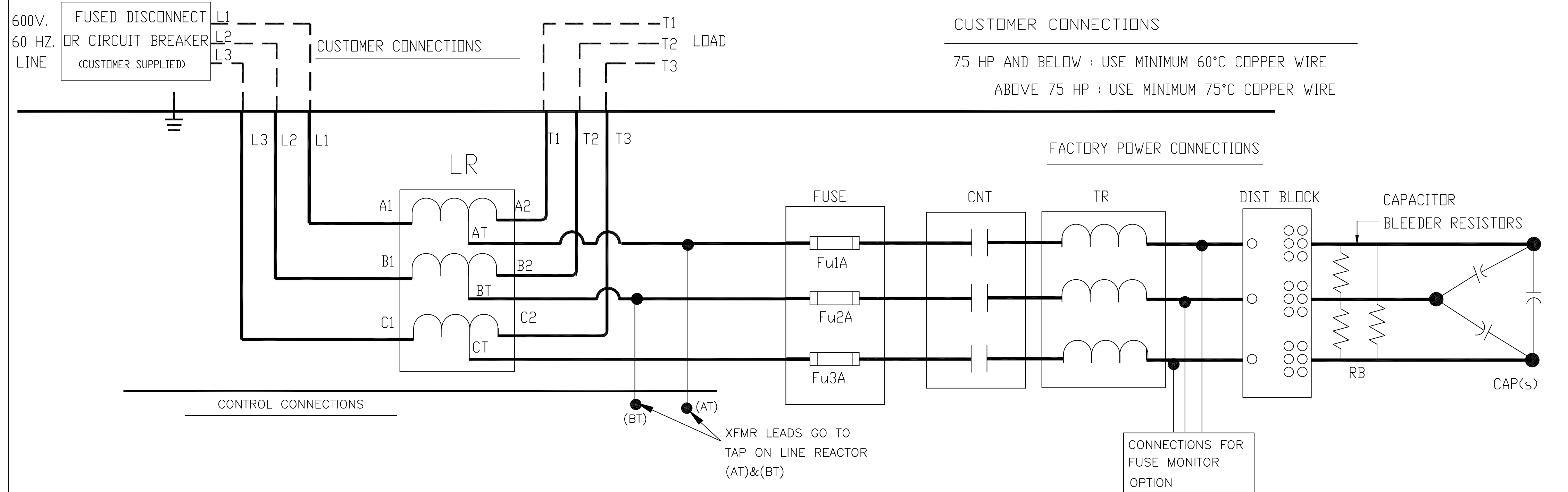
CONTROL CONNECTIONS WITHOUT FAN(S)
