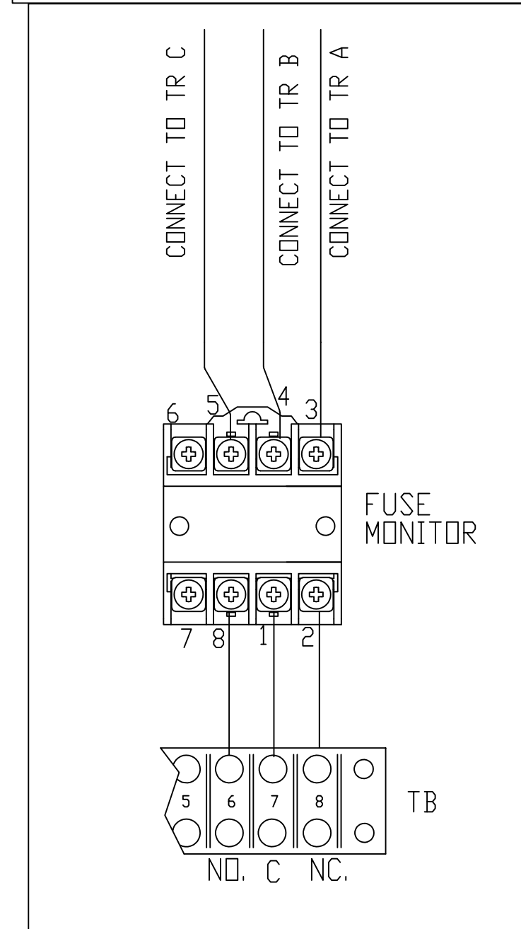
TERMINAL BLOCK ON PANEL
