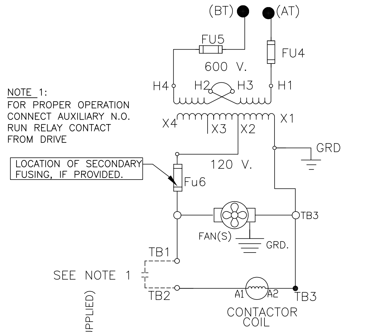
CONTROL CONNECTIONS WITH FAN(S)
