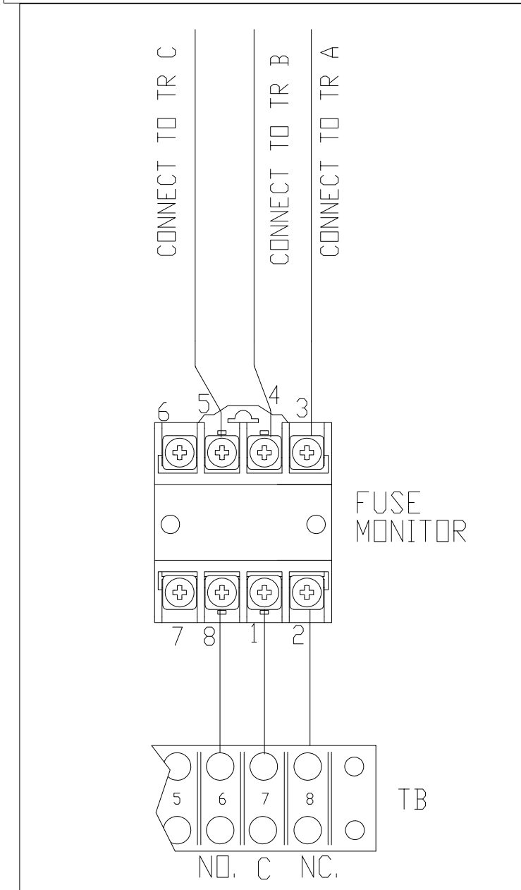
TERMINAL BLOCK ON PANEL
