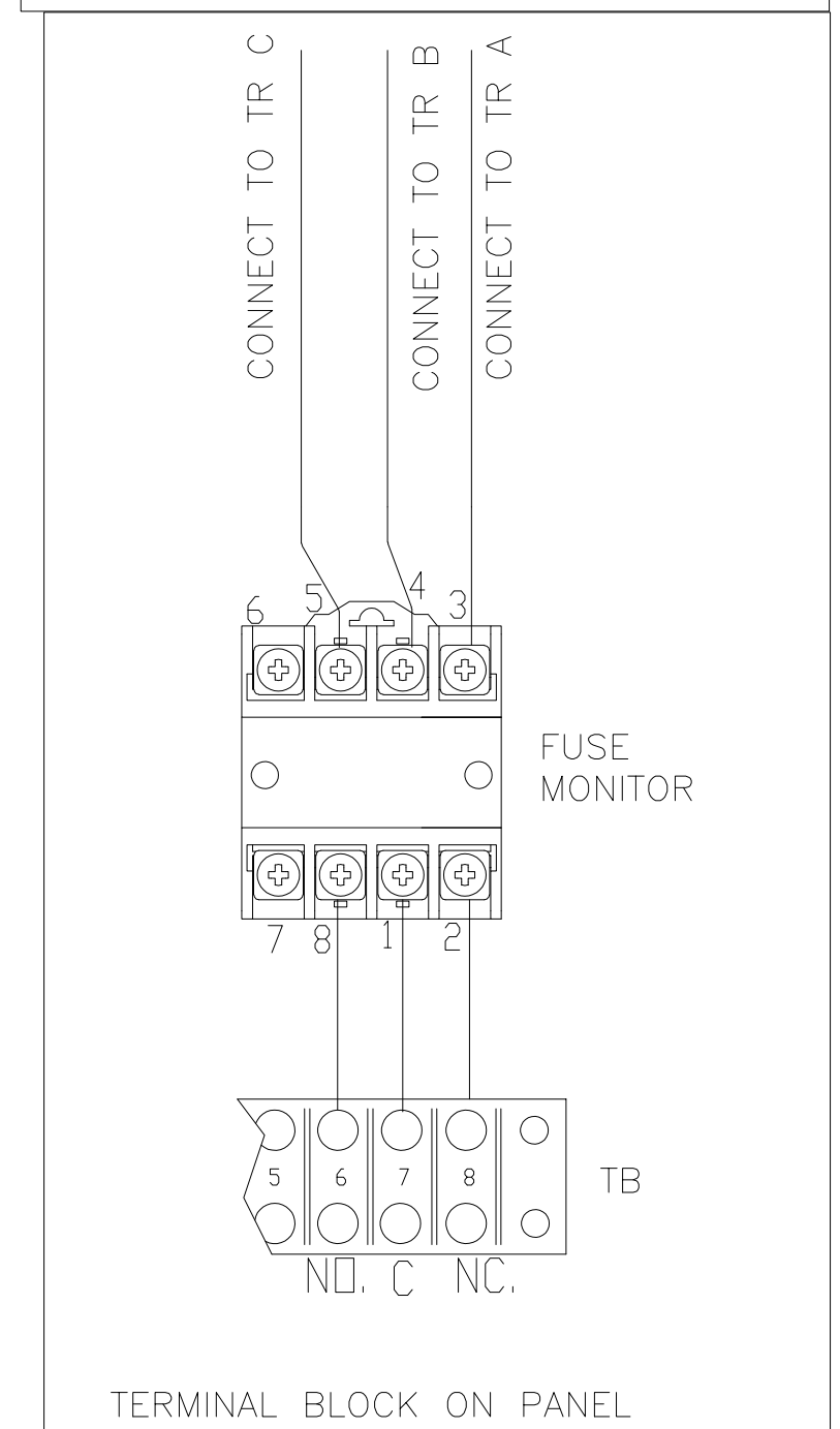
SCHEMATIC FOR FUSE MONITOR, OPTION
