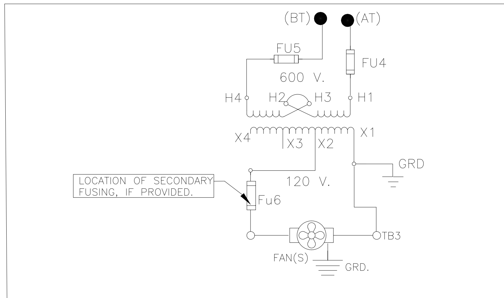
CONTROL CONNECTIONS WITH IF FAN(S) SUPPLIED
