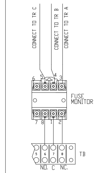
TERMINAL BLOCK ON PANEL
