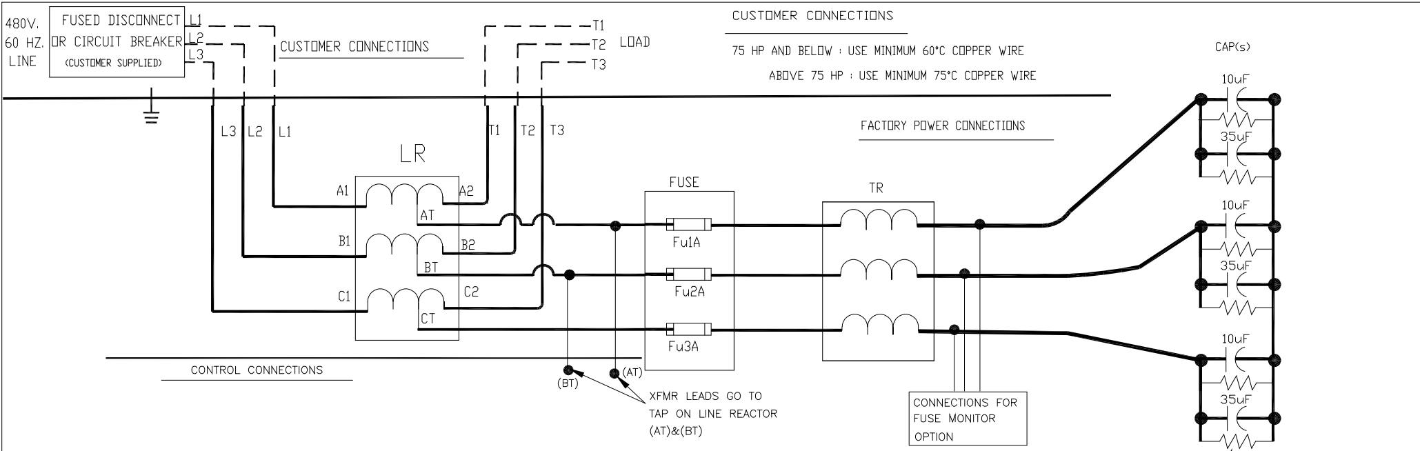
CONTROL CONNECTIONS WITHOUT FAN(S)
