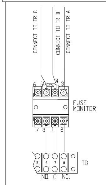
TERMINAL BLOCK ON PANEL
