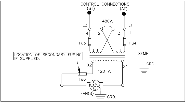
CONTROL CONNECTIONS WITH IF FAN(S) SUPPLIED
