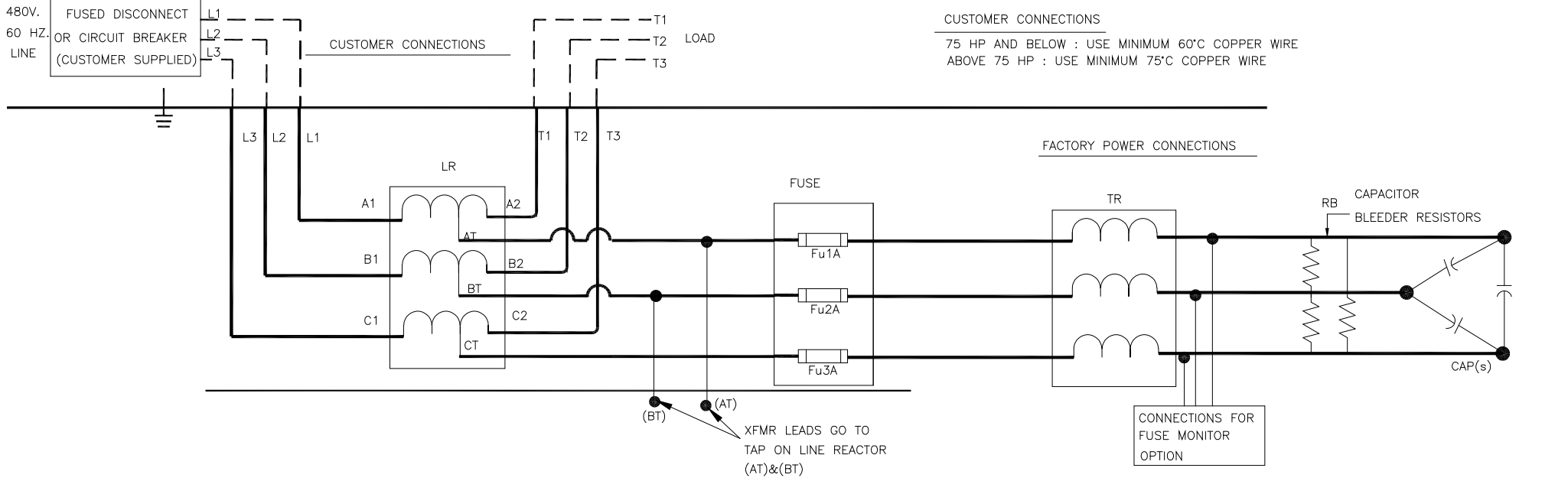
SCHEMATIC FOR FUSE MONITOR, OPTION
