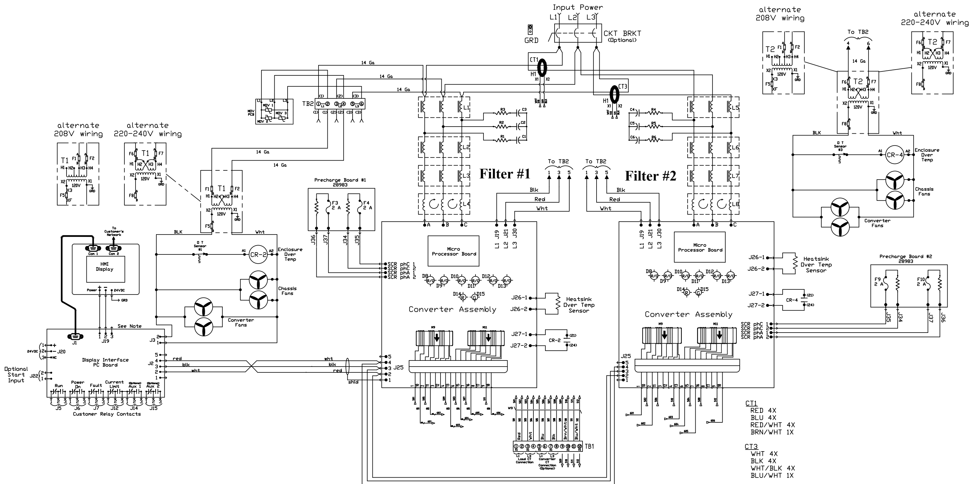
Master/Master Schematic
