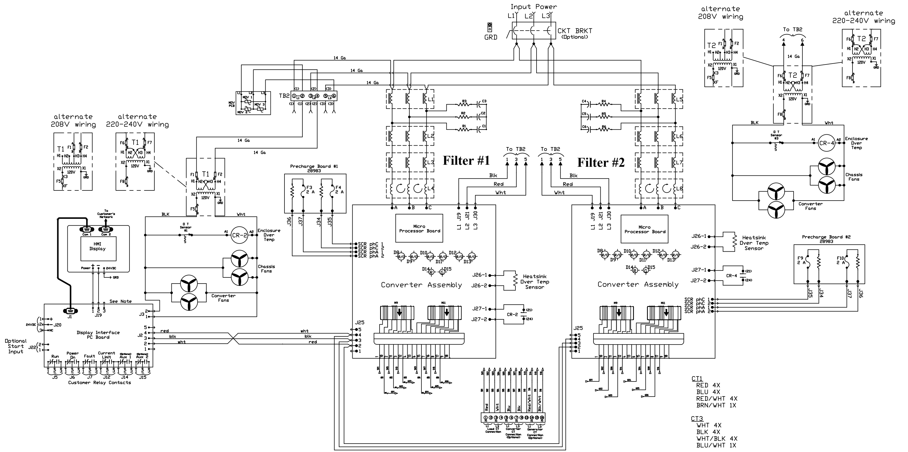
Slave/Slave Schematic
