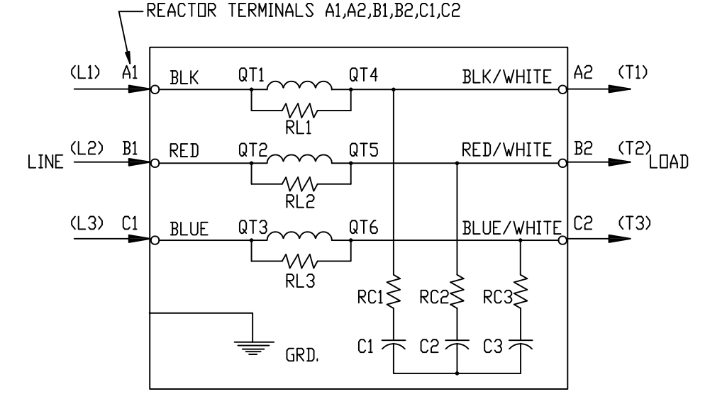
REACTOR AND BOARD ASSEMBLY CONNECTIONS
