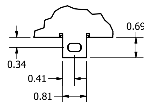
DETAIL B
