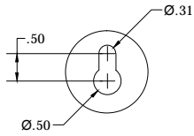
Keyslot × 1 Detail A Scale 2:3
