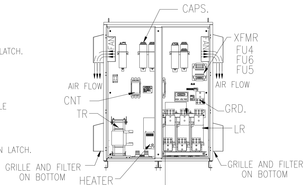
FRONT VIEW WITHOUT DOORS
