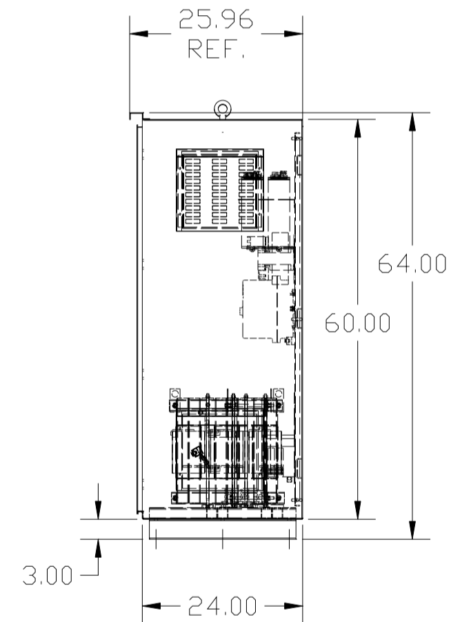
SIDE VIEW
