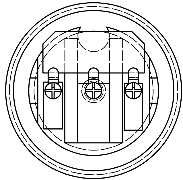
DELTA CONNECTIONS
