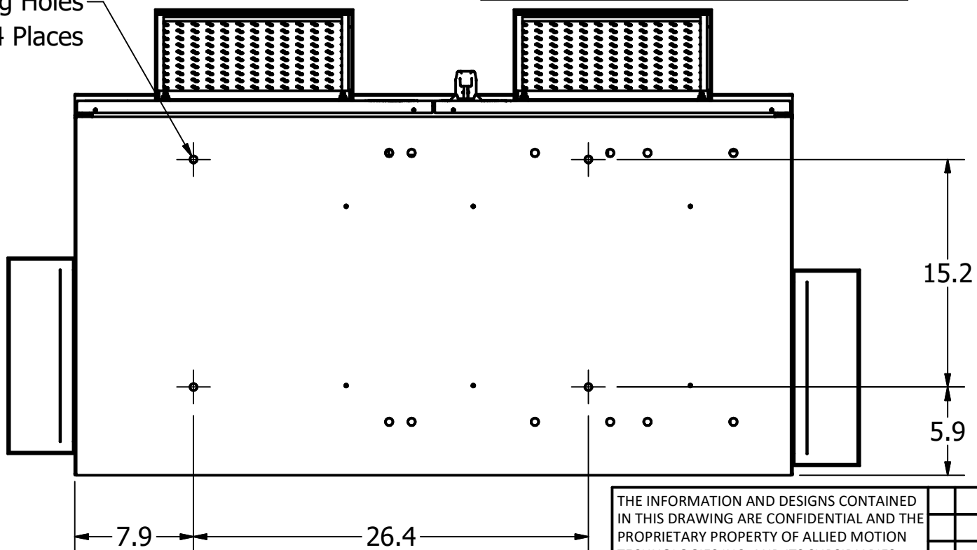
Bottom View
