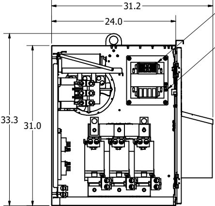
Side View Without Wall
