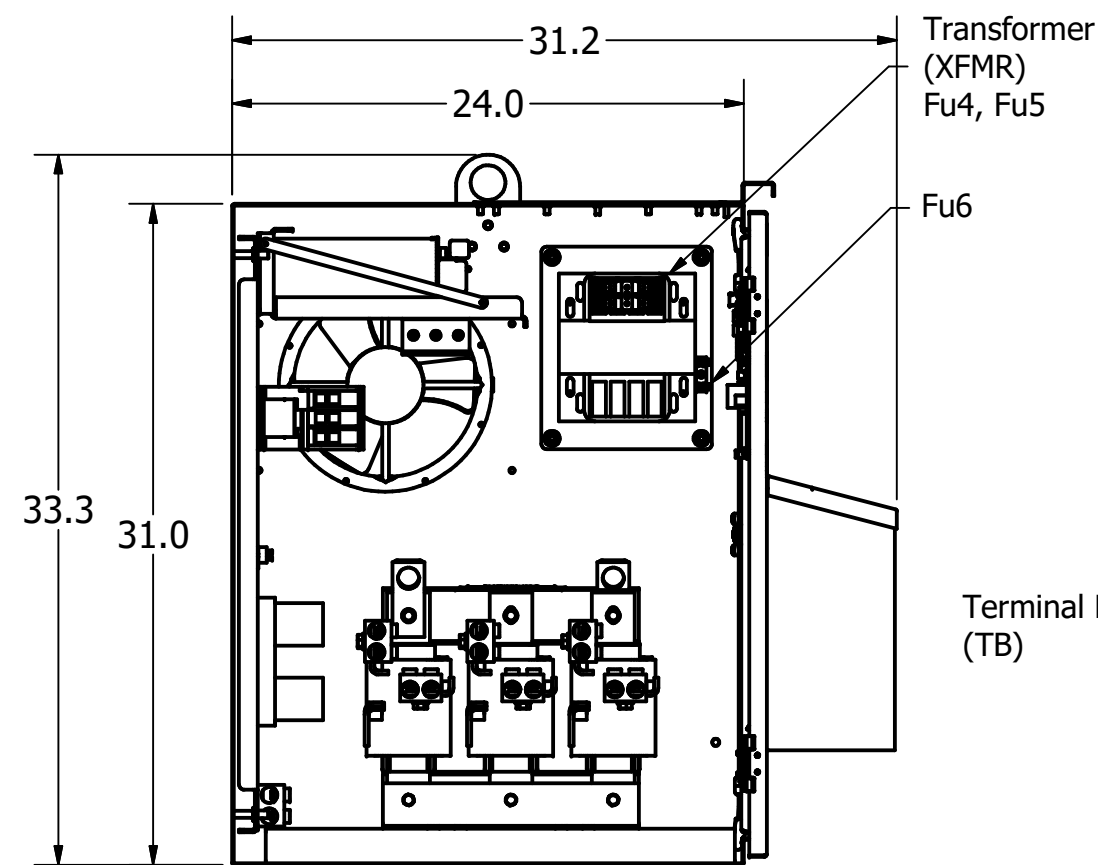
Side View Without Wall
