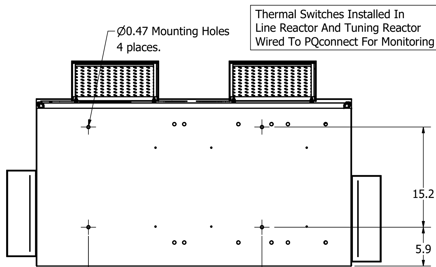
Bottom View
