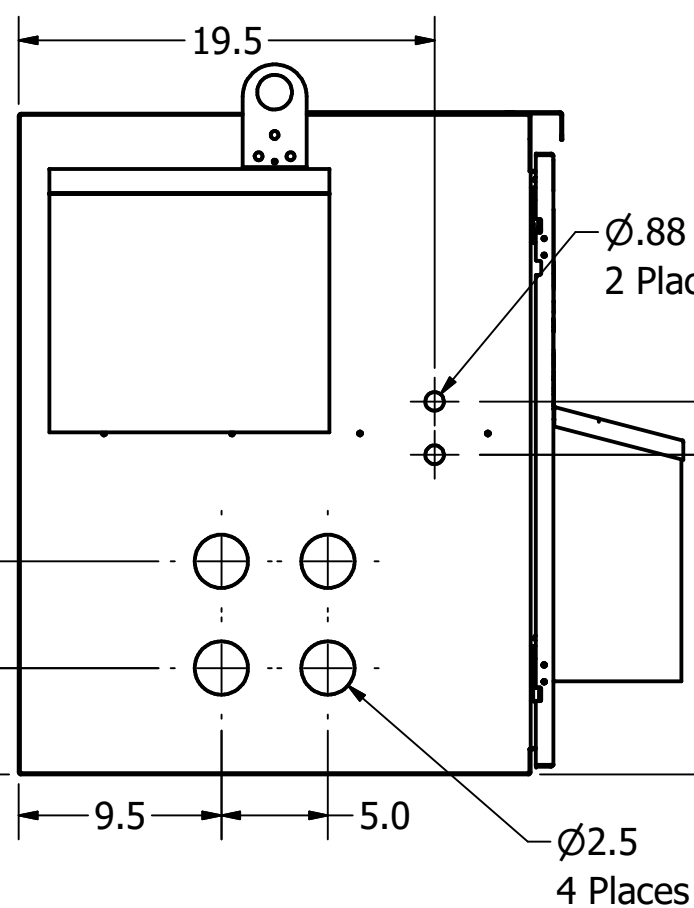
Side View Without Wall
