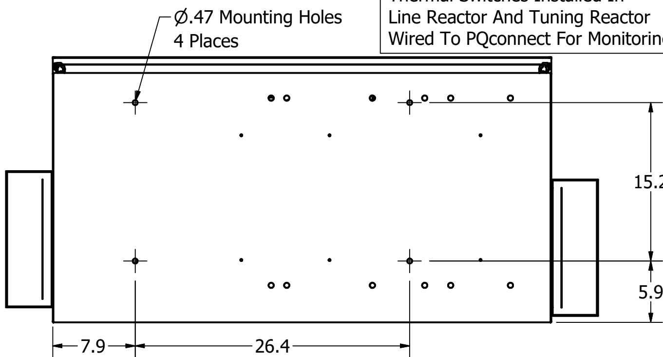
Bottom View
