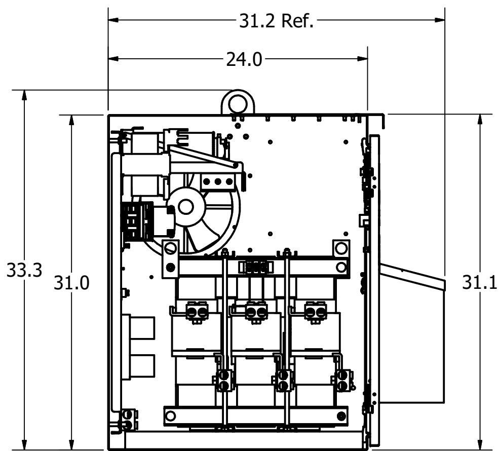
Side View Without Wall
