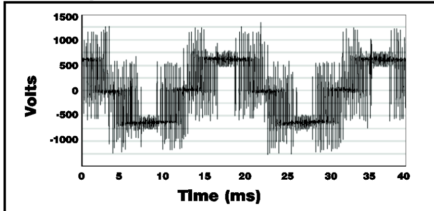
Figure 5.1: Waveform Before MotorShield™
