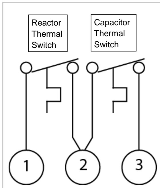
Figure 3.1: Thermal Switches
