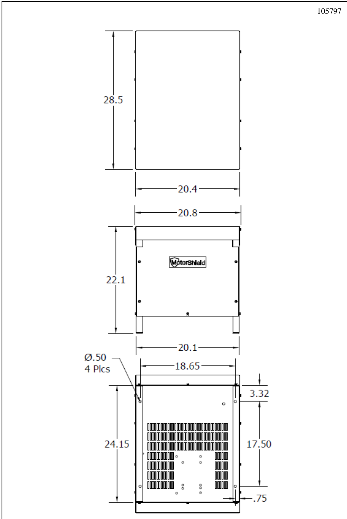
Figure 6.2: MSD 480V, 65A to 130A UL Type 1/3R
