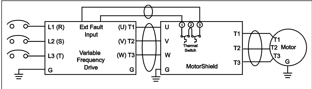
Figure 3.2 – Typical Connection Diagram
