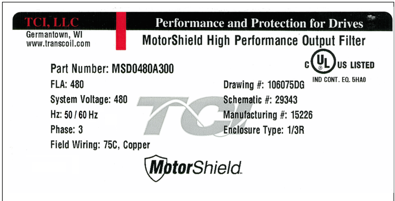
Figure 2.3 – Example of MotorShield™ Nameplate
