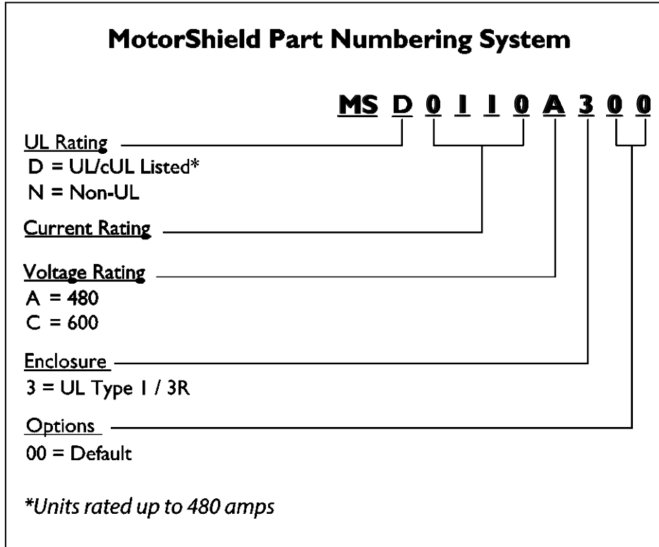
Figure 2.4 – MotorShield™ Model Number Encoding
