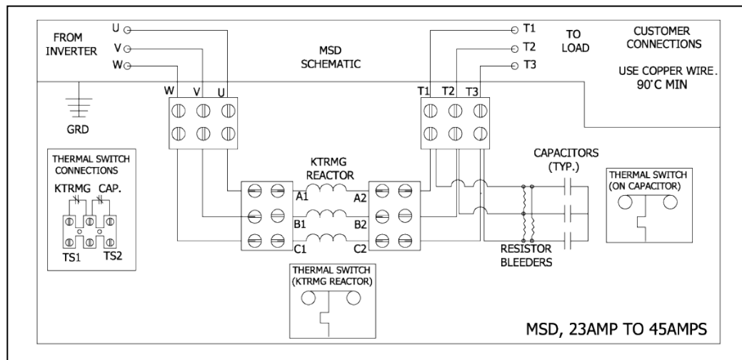
Typical Configuration* for MSD 480V 23A to 45A
