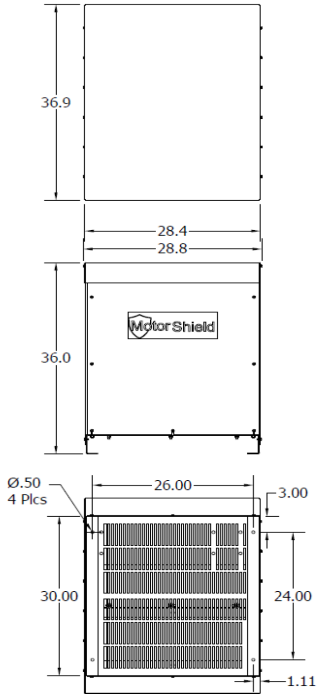
Figure 6.3: MSD 480V, 160A to 480A, UL Type 1/3R
