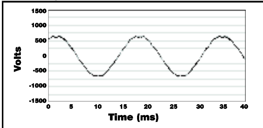
Figure 5.2: Waveform After MotorShield™
