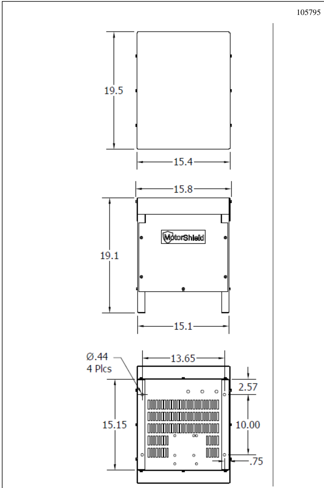
Figure 6.1: MSD 480V 9A to 55A, UL Type 1/3R
